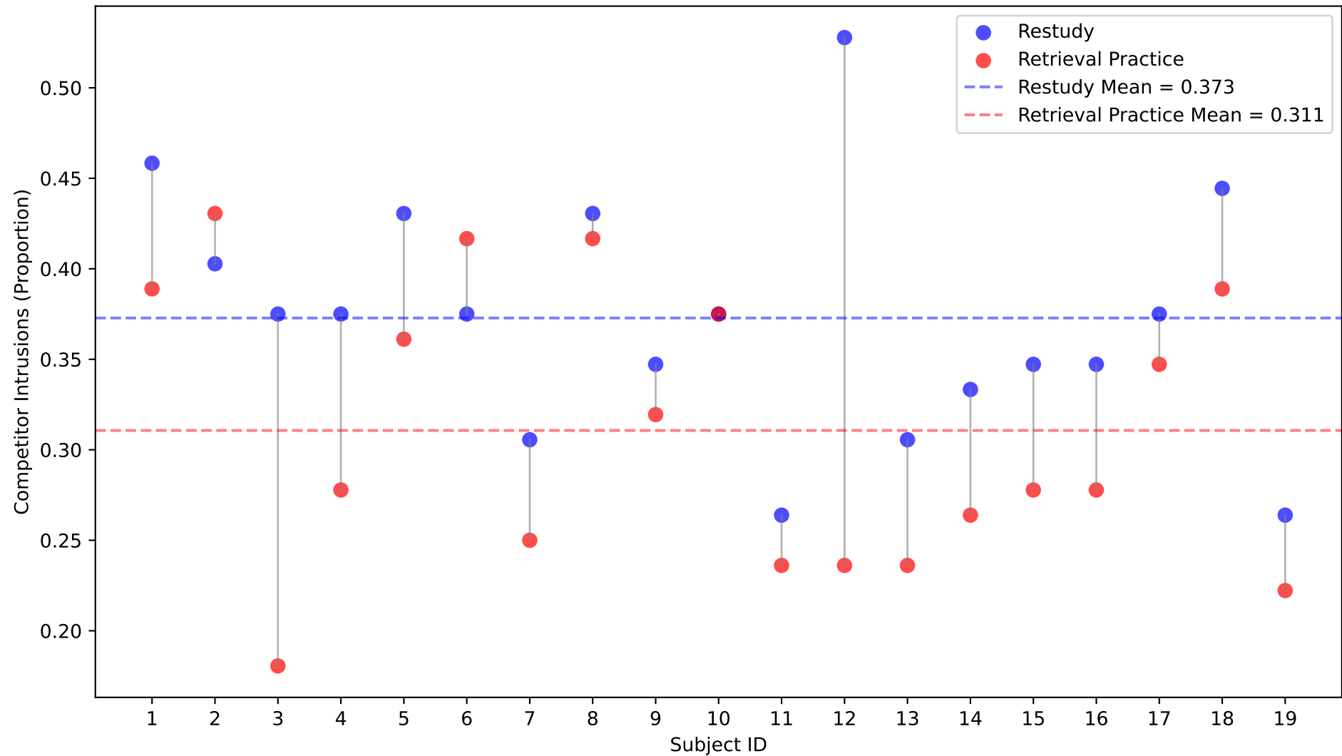
Competitor Intrusions (Proportion): Restudy vs. Retrieval Practice
